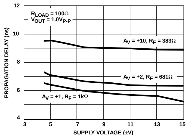
FIGURE 21. PROPAGATION DELAY vs SUPPLY VOLTAGE
