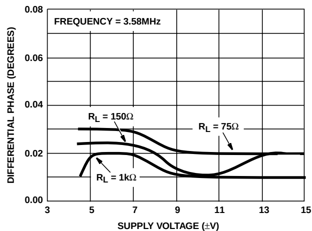
FIGURE 17. DIFFERENTIAL PHASE vs SUPPLY VOLTAGE
