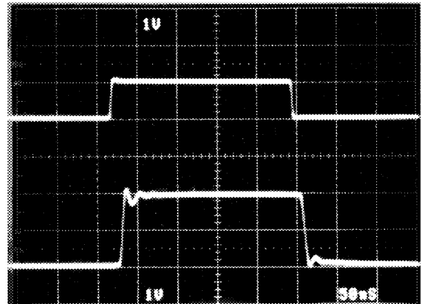
FIGURE 5. LARGE SIGNAL RESPONSE
